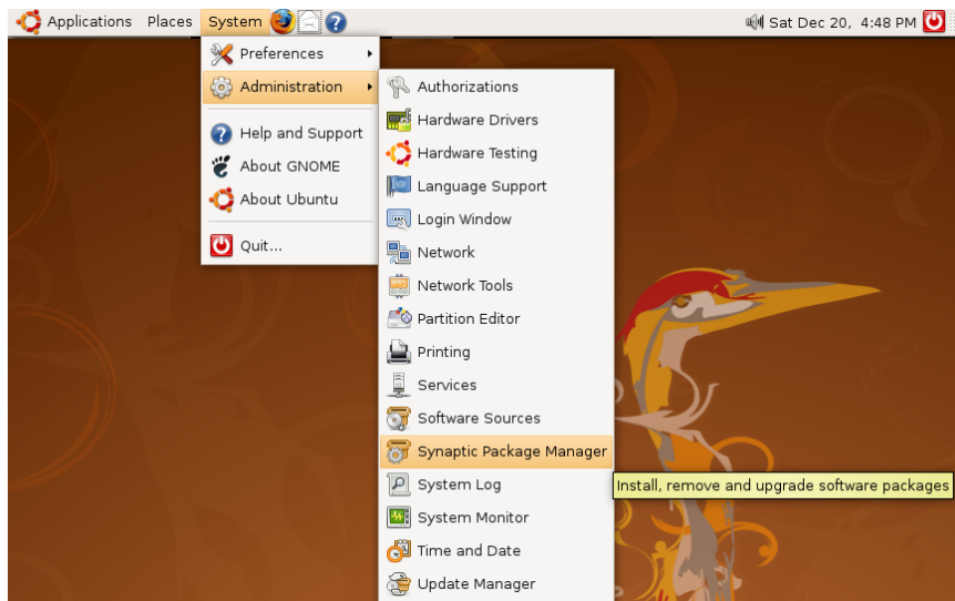
Figure 8.38. Launching Synaptic Package Manager
